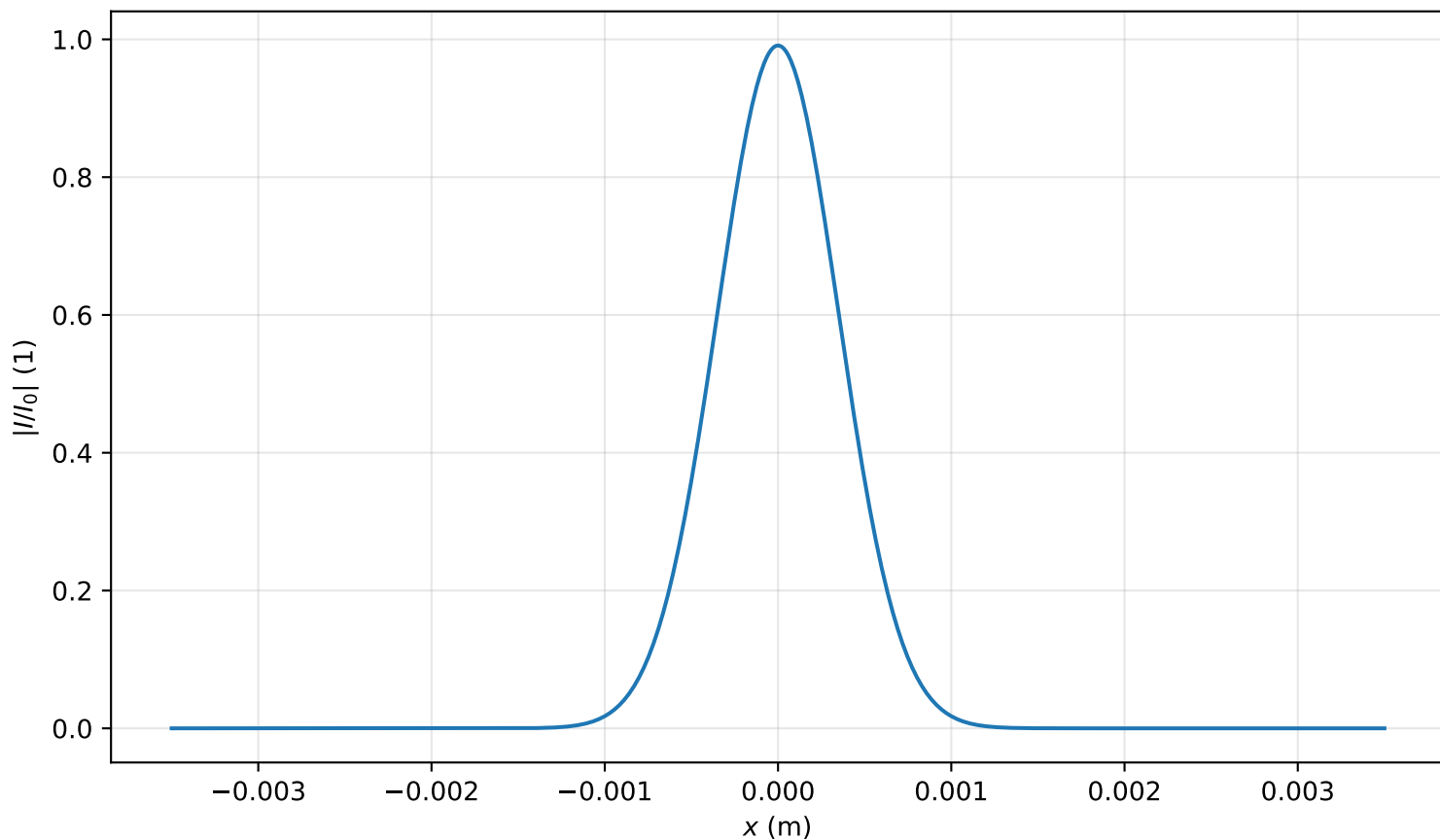
Intensity profile I(x, y = 0, z = 0.239m)/I_0 , P_{in}=0.1P_{cr} , artificial time
